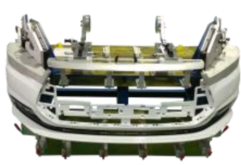
Gauge-Assy plastic part
