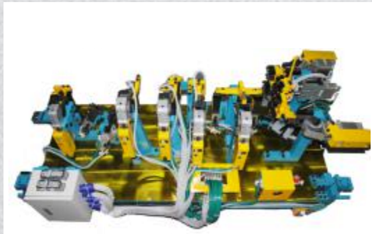
Spot Welding jig
