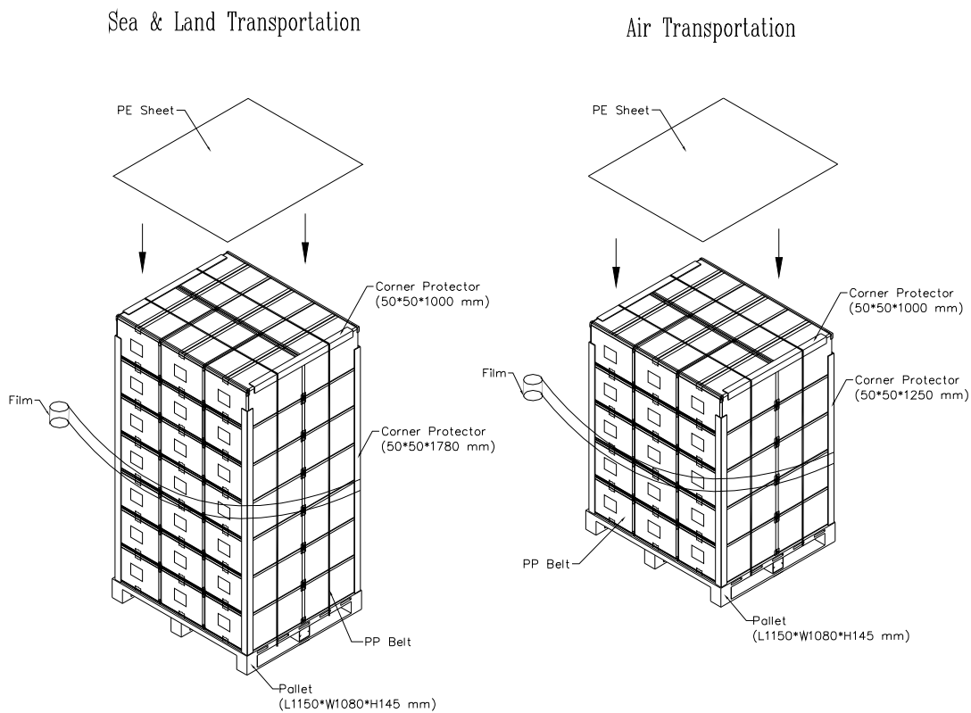
Figure. 7-3 Packing method
