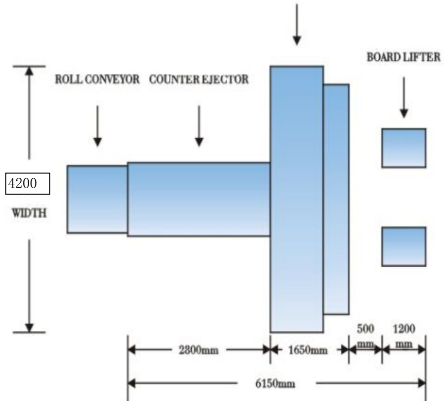
DOUBLE HEADS STITCHER
