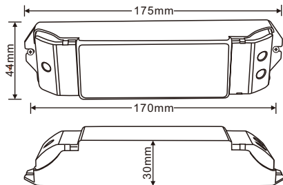
R4-5A/R4-CC Receiver
