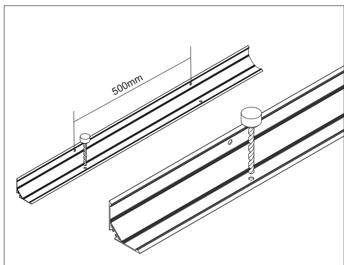
1. Drilling two holes on both sides of profiles with 500mm hole spacings.
