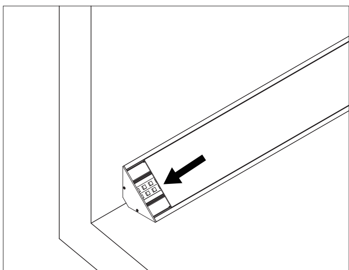
5. Click/snap on the diffuser
