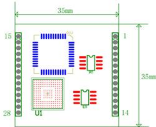
Figure 2 External dimensions of built-in core module (unit: mm)
