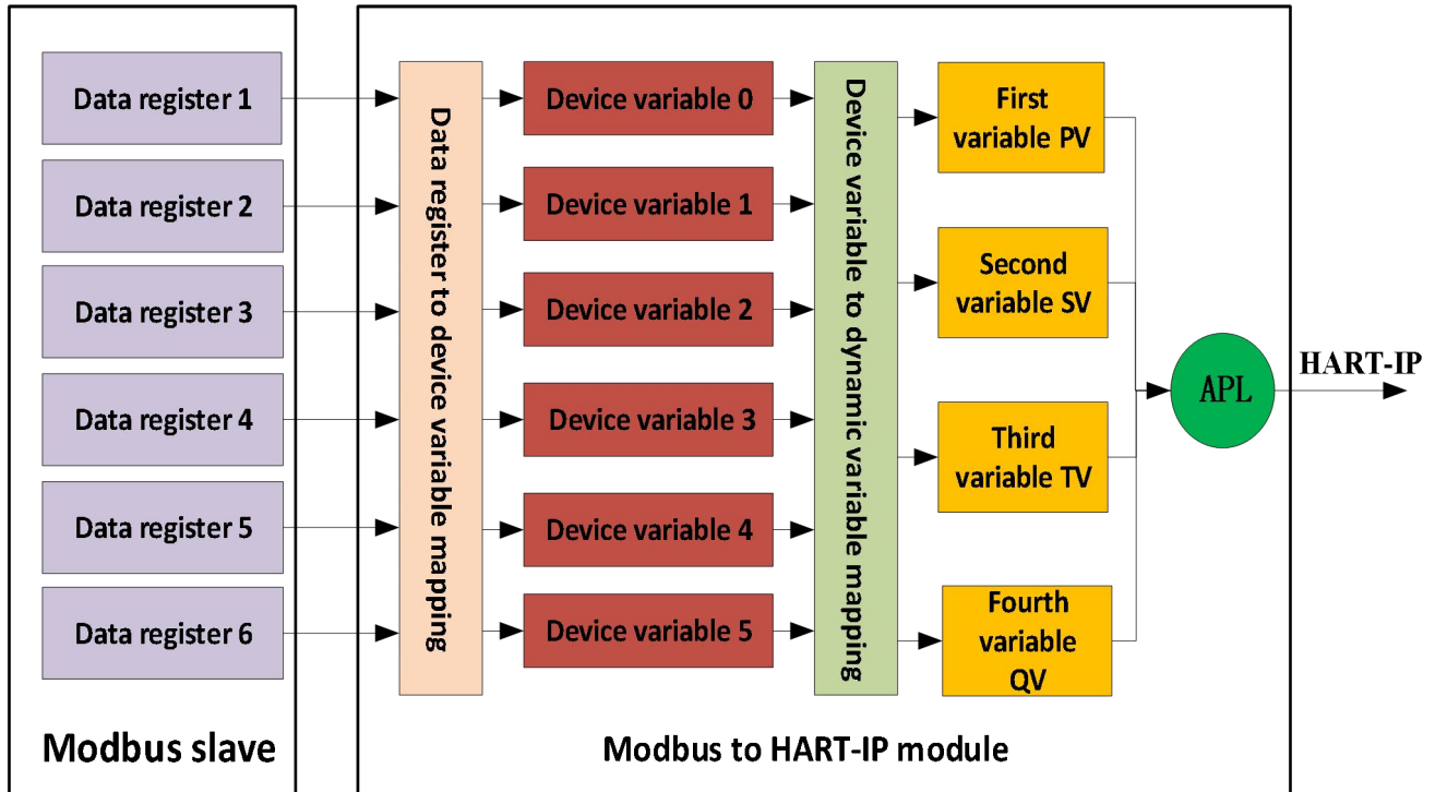
Figure 5 MC0312 data mapping logic diagram
