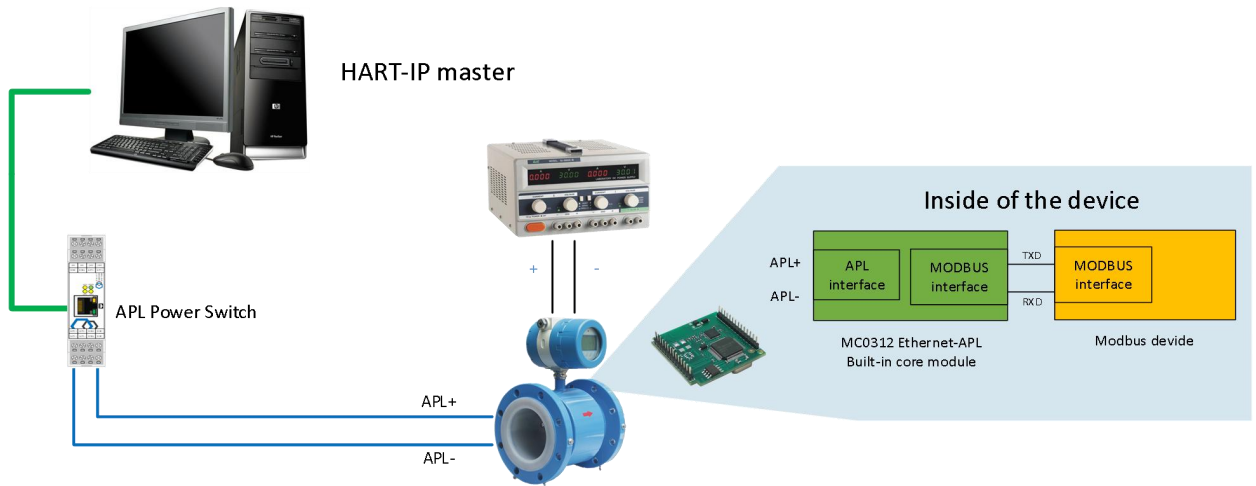
Figure 6 MC0312 module configuration wiring diagram
