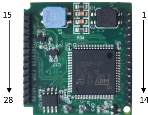
Figure 4 MC0312 built-in core module interface definition
