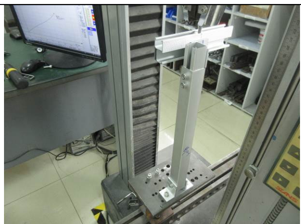
Photo 2: tensile test
