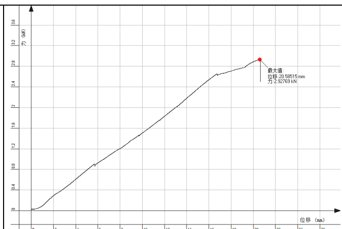
Photo 8: the curve of tension test(3#)
