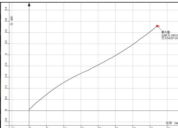
Photo 4: the curve of tension test
