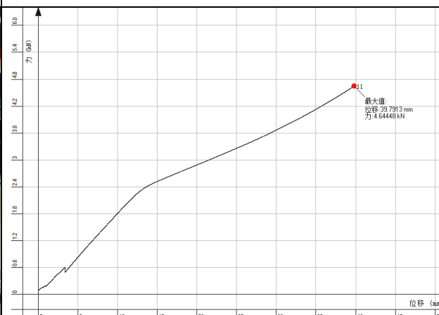
Photo 6: the curve of tension test
