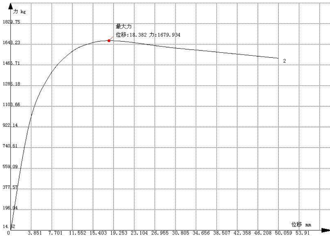
Force-displacement curve
