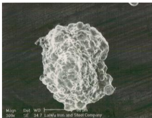
Atomized Iron Powder
