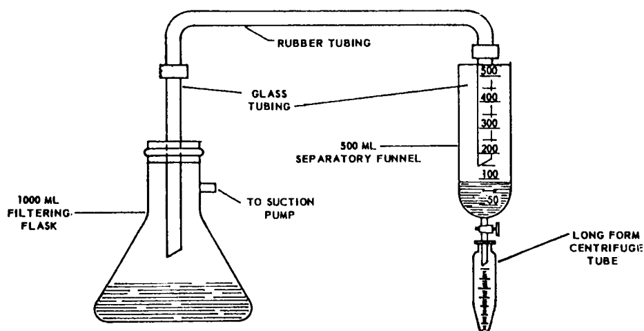
FIG. X1.2 Device to Reduce Volume in Separatory Funnel
