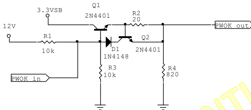
Figure 7.2 Power Ok recommended circuit
