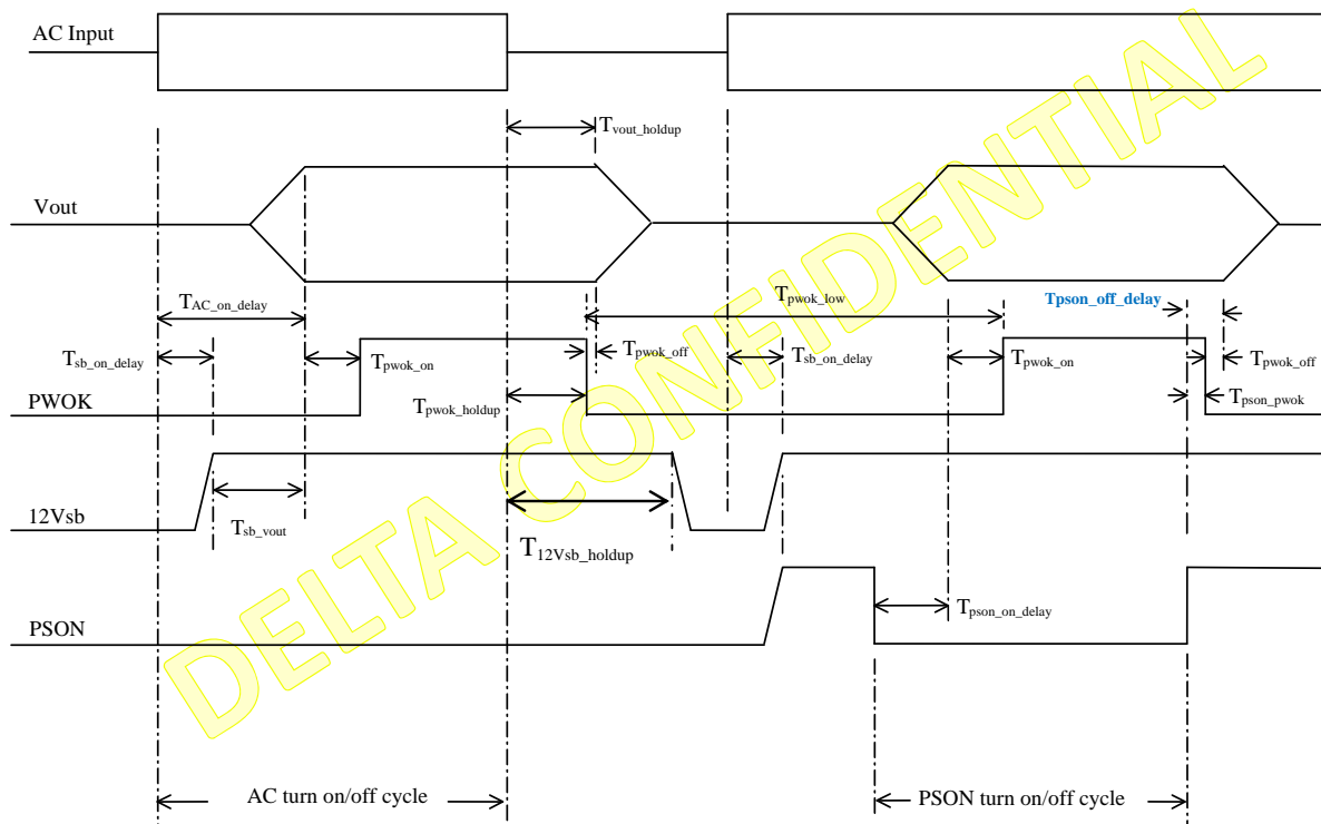
Figure 5.16 Turn On/Off Timing (Power Supply Signals)
