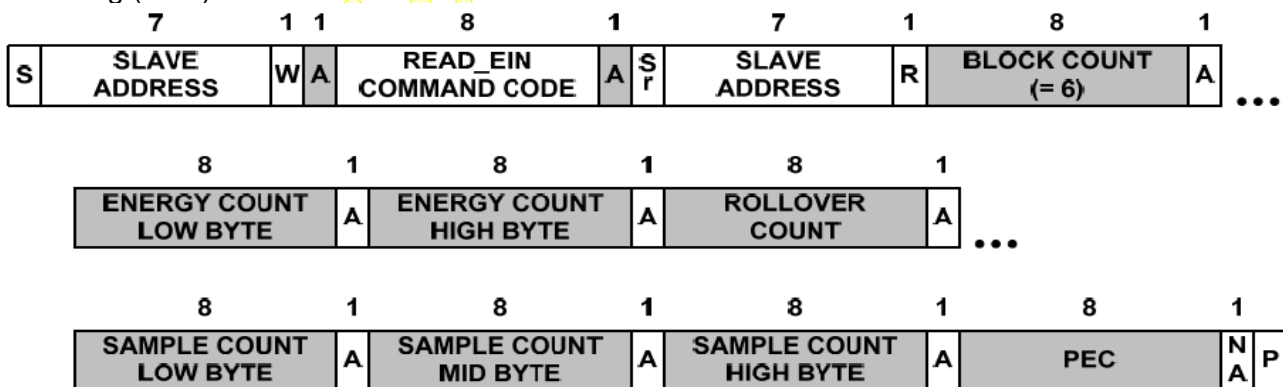
Figure 14.4 READ_EIN Command Packet Format
