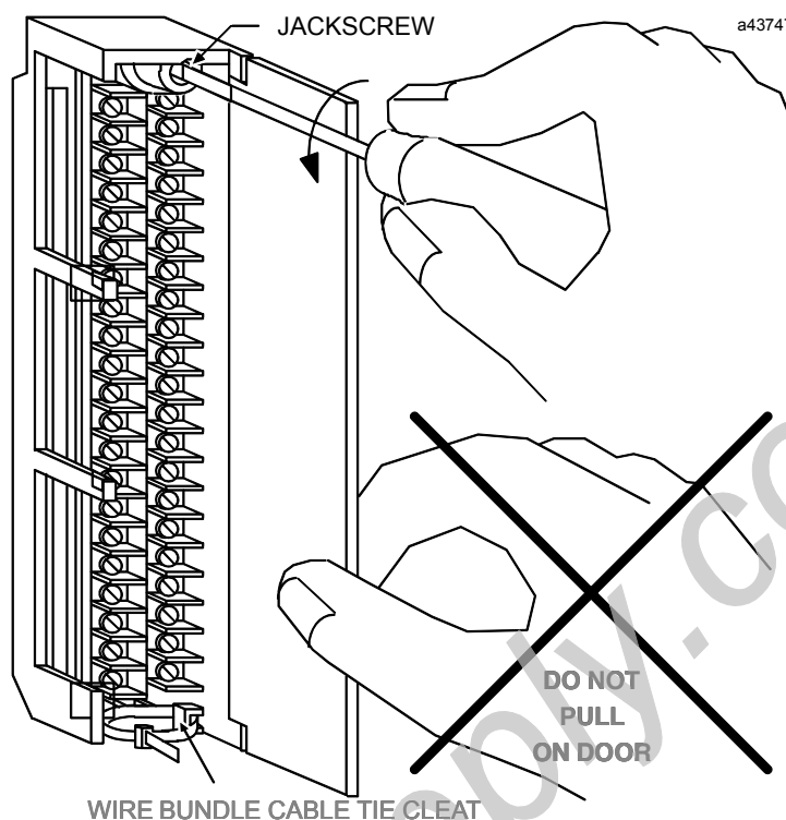
Figure 5. Removal of I/O Terminal Board
