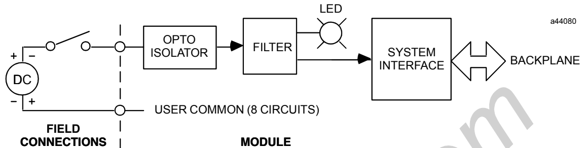
Figure 1. Block Diagram for IC697MDL653
