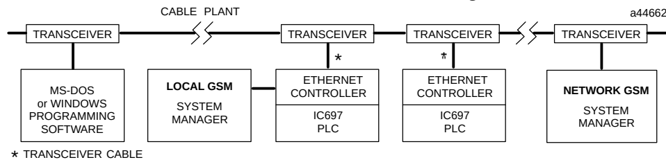
Figure 1. Ethernet Controller Connects the IC697 PLC to a 802.3 LAN
