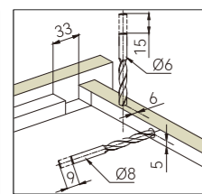
抽屉尺寸和钻孔(mm) Drawer size and drilling
