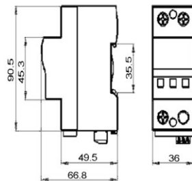
■ Dimension Drawing
