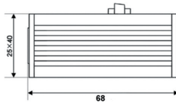
• Dimension drawing
