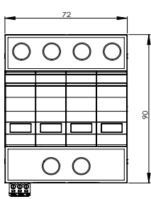
• Dimension drawing
