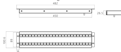
• Dimension drawing
