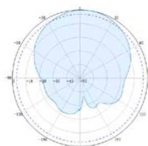
Azimuth(High Band)
