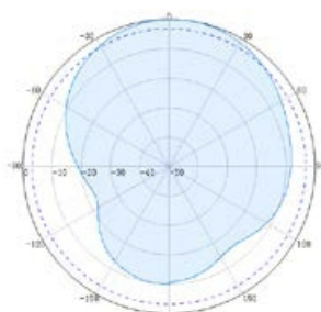
Elevation(Low Band)
