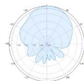
Elevation(High Band)
