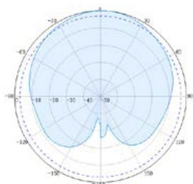
Azimuth(Low Band)
