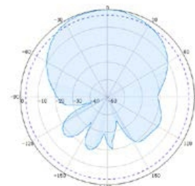
Elevation(High Band)
