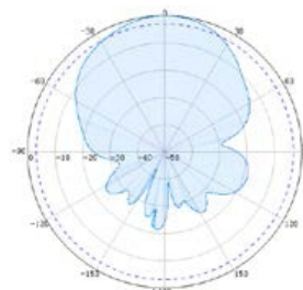
Azimuth(High Band)
