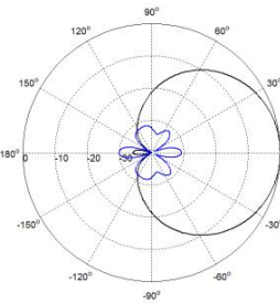
Azimuth(High Band)
