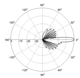
Elevation(High Band)
