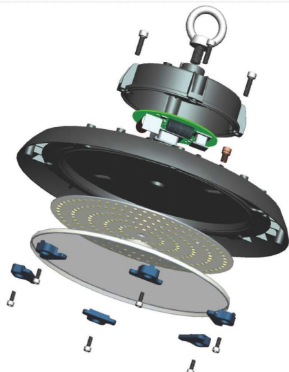
Custom driver internally installed
