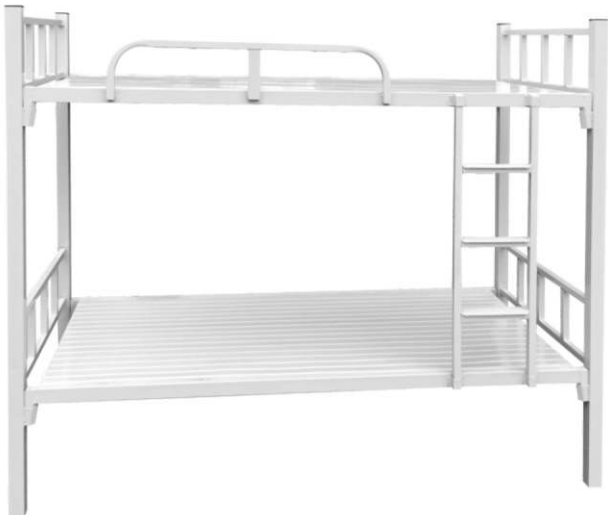
KM-BD-09 L1920xW920xH1700mm
