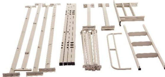
KM-BD-51 L1920xW920xH1800mm
