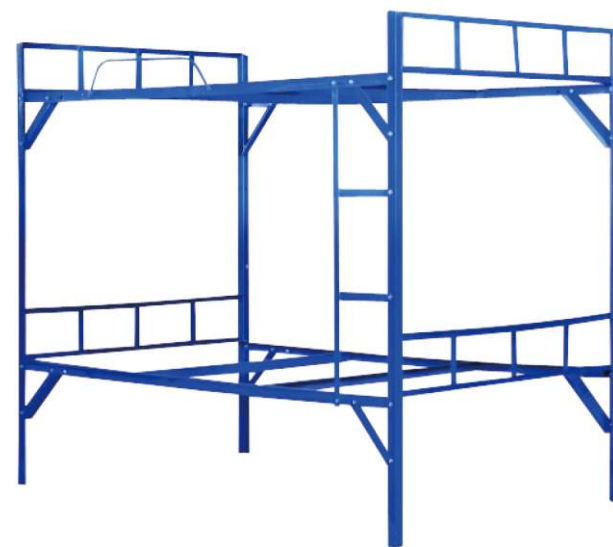
KM-BD-38 L1920xW920xH1600mm
