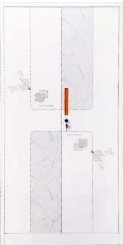
KM-WD-18 Wardrobe 两门衣柜 H1850xW900xD450mm
