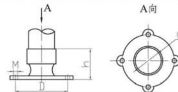
管形母线终端固定金具 (MGD型) Tubular Bus-bar End Supports (Type MGD)
