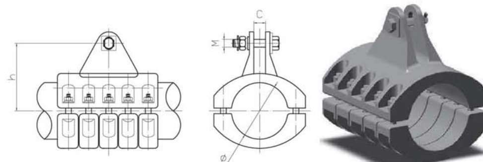
悬吊式管母线固定金具 (MGXX2型直吊式) Suspension Supports for Tubular Bus-bar (Type MGXX2, Vertical Type)
