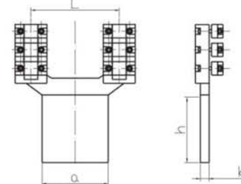
双导线设备线夹 (0° SSL螺栓型) Terminal Clamps For Double-Bundle Conductor (Type SSL)
