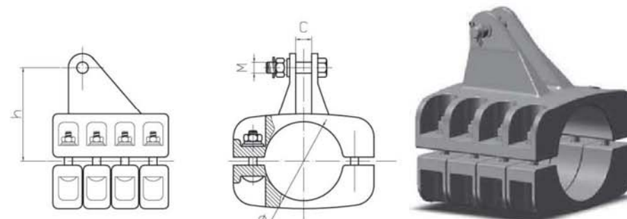
悬吊式管母线固定金具 (MGXX1型斜吊式) Suspension Supports for Tubular Bus-bar (Type MGXX1, Oblique Type)
