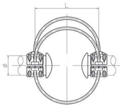
管母线伸缩金具 (MGSD (L) 型) Tubular Bus-bar Flexible Fittings (Type MGSD/L)
