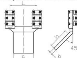
导线设备线夹 (45° SSL螺栓型) Terminal Clamps For Double-Bundle Conductor (Type SSL)
