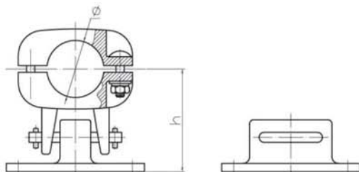
管形母线固定金具 (MGG1滑动型) Tubular Bus-bar Supports (Type MGG1)
