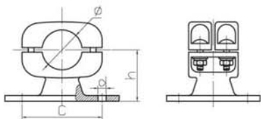
管形母线固定金具 (MGG型) Tubular Bus-bar Supports (Type MGG)
