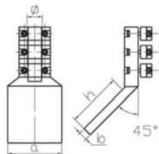
大截面导线设备线夹 (45° SL螺栓型) Terminal Clamps For Single-Conductor (Type SL)
