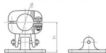
管形母线固定金具 (MGG2摆动型) Tubular Bus-bar Supports (Type MGG2)
