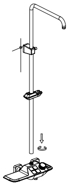
5.Rotate the shower tube assembly to the main body, and then mark the fixed seat position.
