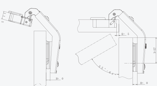
ART.NO. 813135 (Clip on soft close hinge)
