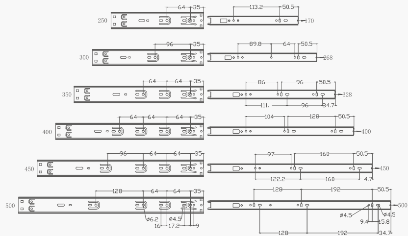
Screw position of slide(mm)
