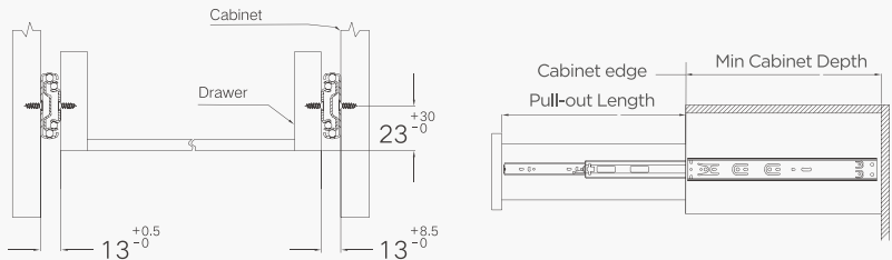
Installation dimension
