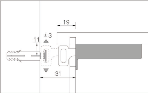
Suspension hook dimension
