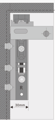
Suspension hook dimension
