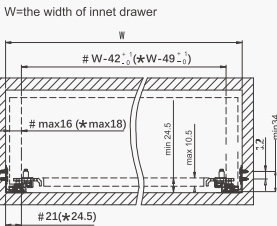
Installation dimension(mm)
