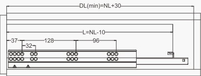
Installation for standard drawer
