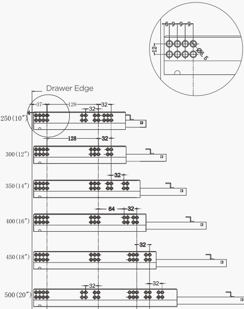
Screw position of the slide(mm) Unit:mm
