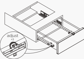
Drawer adjustment
