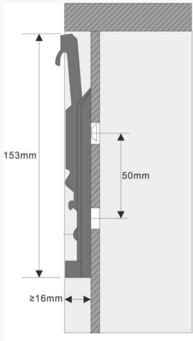
Installation dimension
