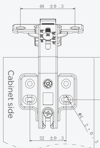
ART.NO. 813134 (Slide on soft close hinge)
