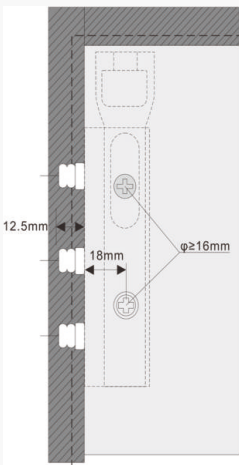
Drilling distance
