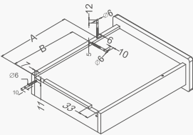
Drawer Back Preparation(mm)
