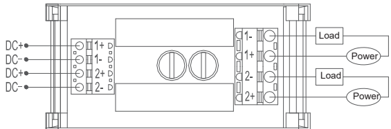
DRA-2-KSF/ KSLE Series Wiring Diagram
