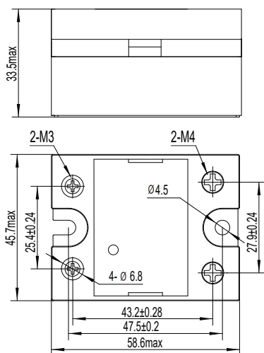
Current Control
