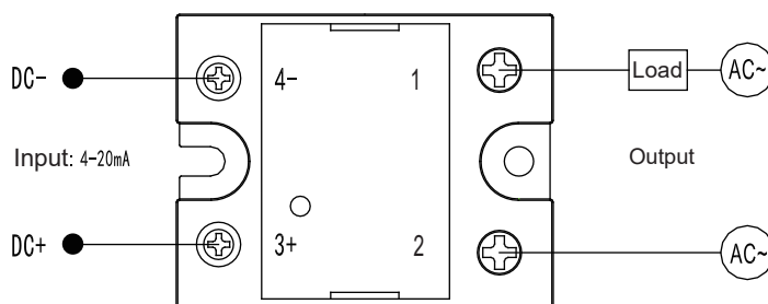
Current Control
