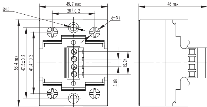
Outline Dimensions
