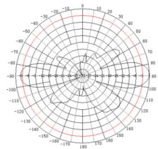
5G E Plane
