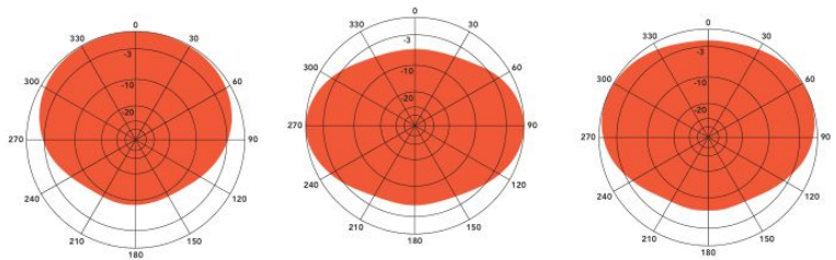
H-plane:Gain9.1dBd
