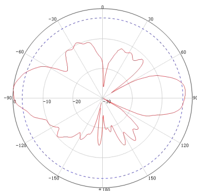
Typical pattern E Plane
