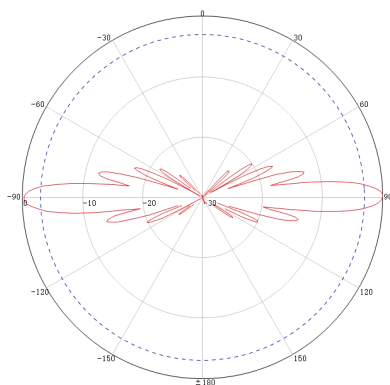
Typical pattern E Plane
