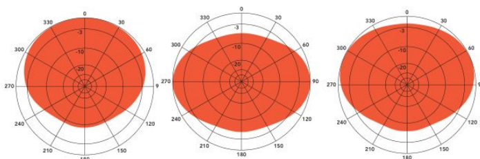
H-plane:Gain11.2dBi H-plane:Gain11.2dBi H-plane:Gain10.6dBi 1/4 \lambda .spacing from tower 1/2 \lambda .spacing from tower 3/8 \lambda .spacing from tower
