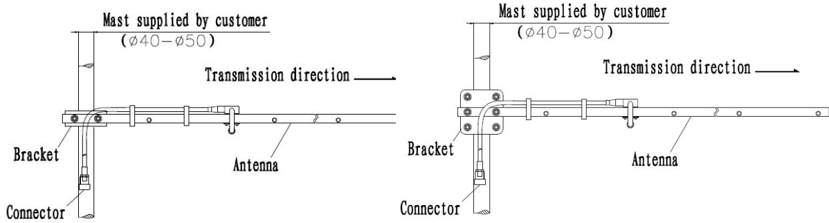
3/5/7/9 Unit Installation Sketch
