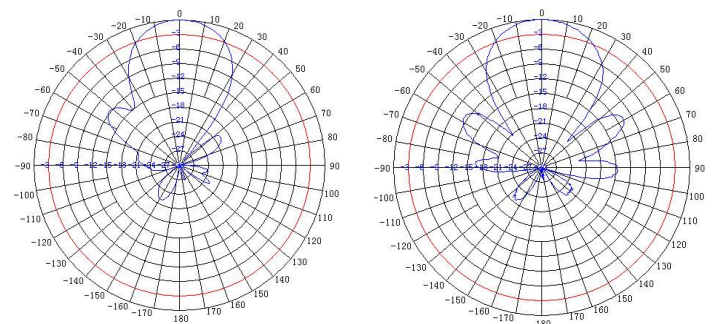
E Plane
