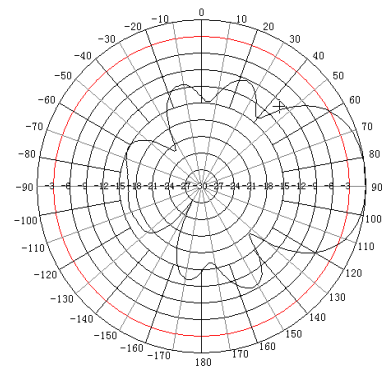
H Plane
