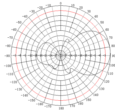
E Plane
