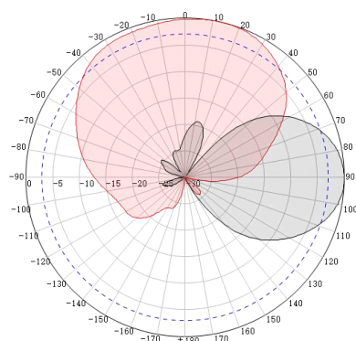
Radiation pattern 2.4GHz
