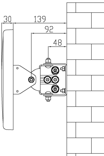
Installation Sketch
