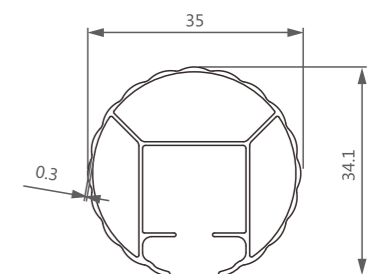
型号/Item No.-151409 米重/Weight-0.307kg/m
