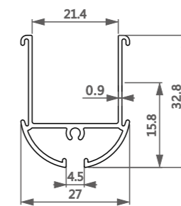
型号/Item No.-1116540 米重/Weight-0.318kg/m
