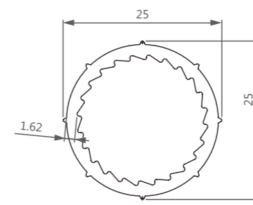
型号/Item No.-111101 米重/Weight-0.381kg/m
