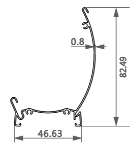
型号/Item No.-1118384 米重/Weight-0.484kg/m
