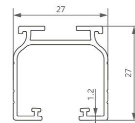
型号/Item No.-13031422 米重/Weight-0.351kg/m
