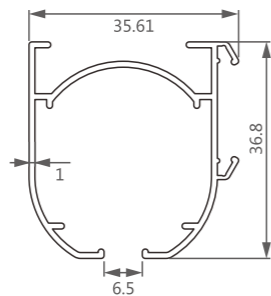
型号/Item No.-1514355 米重/Weight-0.403kg/m
