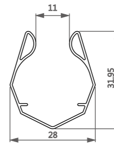
型号/Item No.-11181443 米重/Weight-0.217kg/m
