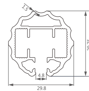
型号/Item No.-13031423 米重/Weight-0.571kg/m
