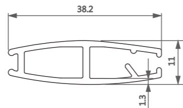
型号/Item No.-11181651 米重/Weight-0.365kg/m
