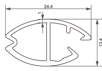
型号/Item No.-1118978 米重/Weight-0.217kg/m
