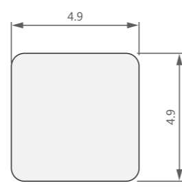
型号/Item No.-151401 米重/Weight-0.065kg/m
