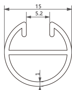
型号/Item No.-1116099 米重/Weight-0.152kg/m
