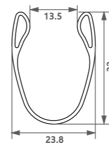
型号/Item No.-11181766 米重/Weight-0.271kg/m
