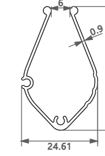
型号/Item No.-11182093 米重/Weight-0.275kg/m
