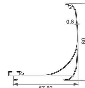
型号/Item No.-11182094 米重/Weight-0.535kg/m
