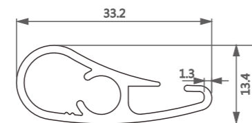
型号/Item No.-1118695 米重/Weight-0.298kg/m
