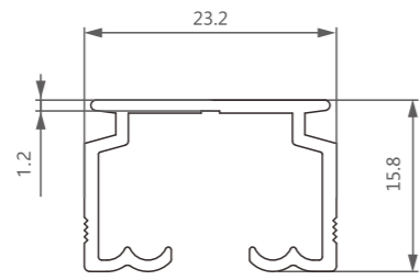
型号/Item No.-13031323 米重/Weight-0.226kg/m
