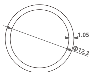
型号/Item No.-6110276 米重/Weight-0.120kg/m
