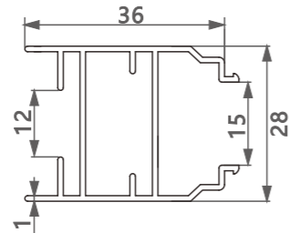
型号/Item No.-13031242 米重/Weight-0.435kg/m
