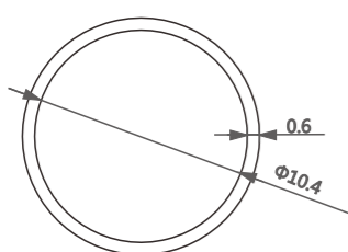
型号/Item No.-6110366 米重/Weight-0.057kg/m
