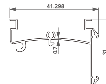
型号/Item No.-111368 米重/Weight-0.242kg/m
