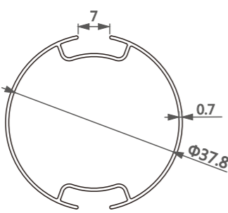
型号/Item No.-1116577 米重/Weight-0.279kg/m
