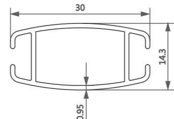
型号/Item No.-11161181 米重/Weight-0.234kg/m
