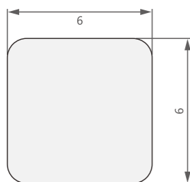
型号/Item No.-151417 米重/Weight-0.097kg/m
