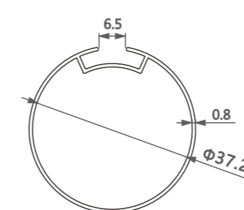
型号/Item No.-110123-0.8 米重/Weight-0.292kg/m
