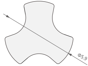
型号/Item No.-1303169 米重/Weight-0.050kg/m
