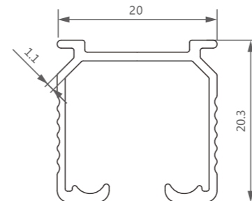
型号/Item No.-1303844 米重/Weight-0.204kg/m
