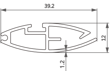
型号/Item No.-1116433 米重/Weight-0.331kg/m
