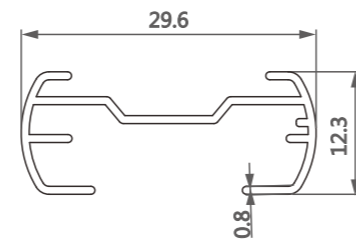
型号/Item No.-1514681 米重/Weight-0.165kg/m
