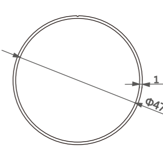
型号/Item No.-11161265-1.0 米重/Weight-0.411kg/m
