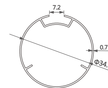
型号/Item No.-110110 米重/Weight-0.246kg/m
