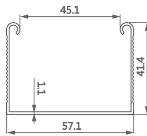
型号/Item No.-1202277 米重/Weight-0.424kg/m
