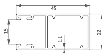
型号/Item No.-79081017 米重/Weight-0.465kg/m
