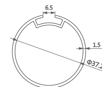
型号/Item No.-110123-1.5 米重/Weight-0.53kg/m
