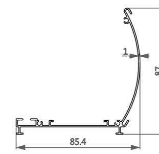
型号/Item No.-1116955 米重/Weight-0.618kg/m
