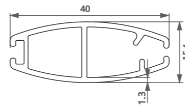
型号/Item No.-1116649 米重/Weight-0.401kg/m
