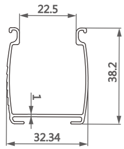
型号/Item No.-1202475 米重/Weight-0.328kg/m
