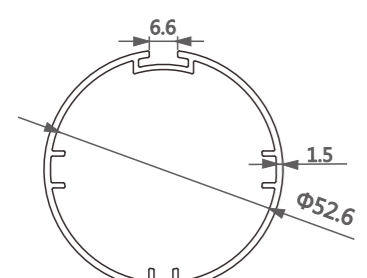
型号/Item No.-1116333-1.5 米重/Weight-0.789kg/m
