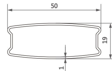
型号/Item No.-11161547 米重/Weight-0.348kg/m
