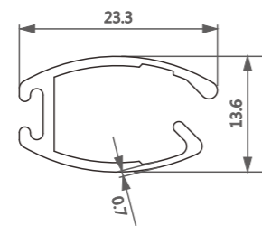
型号/Item No.-191071 米重/Weight-0.190kg/m
