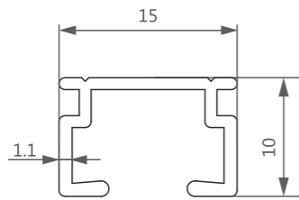
型号/Item No.-1303201 米重/Weight-0.120kg/m
