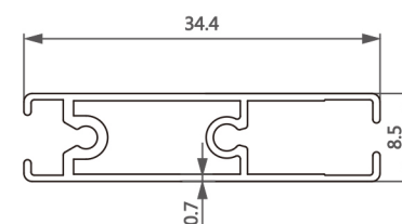
型号/Item No.-1907243-0.7 米重/Weight-0.199kg/m
