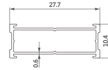
型号/Item No.-11181333 米重/Weight-0.141kg/m
