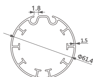
型号/Item No.-1118911 米重/Weight-1.270kg/m
