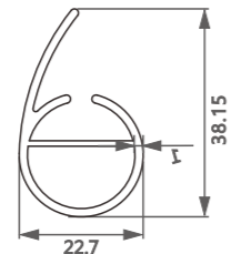
型号/Item No.-111827 米重/Weight-0.408kg/m
