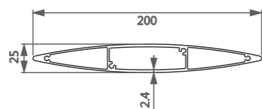
型号/Item No.-42371268 米重/Weight-2.405kg/m
