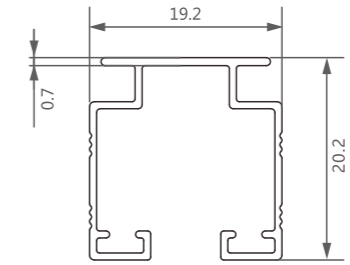
型号/Item No.-13031308 米重/Weight-0.162kg/m
