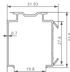
型号/Item No.-1514915 米重/Weight-0.248kg/m
