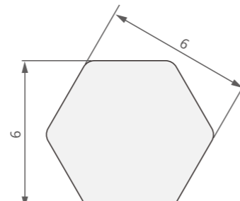
型号/Item No.-191137 米重/Weight-0.085kg/m
