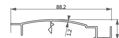
型号/Item No.-19070541 米重/Weight-0.452kg/m
