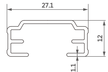
型号/Item No.-1514239 米重/Weight-0.197kg/m
