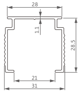
型号/Item No.-1303163 米重/Weight-0.311 kg/m
