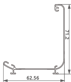
型号/Item No.-11181739 米重/Weight-0.426kg/m
