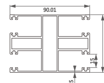
型号/Item No.-0901509 米重/Weight-2.55kg/m
