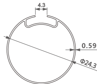
型号/Item No.-11161098 米重/Weight-0.144kg/m
