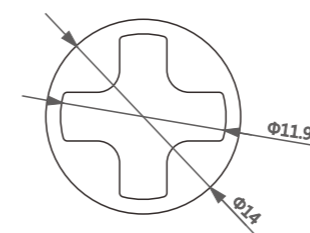
型号/Item No.-1116078 米重/Weight-0.226kg/m
