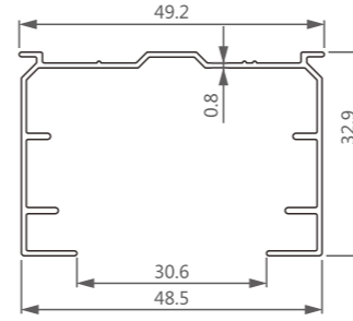
型号/Item No.-1514170 米重/Weight-0.341 kg/m
