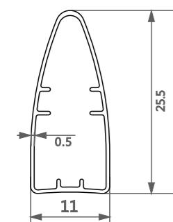
型号/Item No.-11161063 米重/Weight-0.101kg/m
