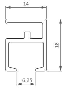
型号/Item No.-1514858 米重/Weight-0.198kg/m
