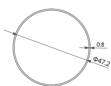
型号/Item No.-6110382-0.8 米重/Weight-0.330kg/m
