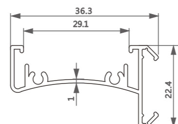
型号/Item No.-1116191 米重/Weight-0.316kg/m
