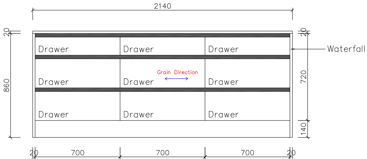
Elevation C
