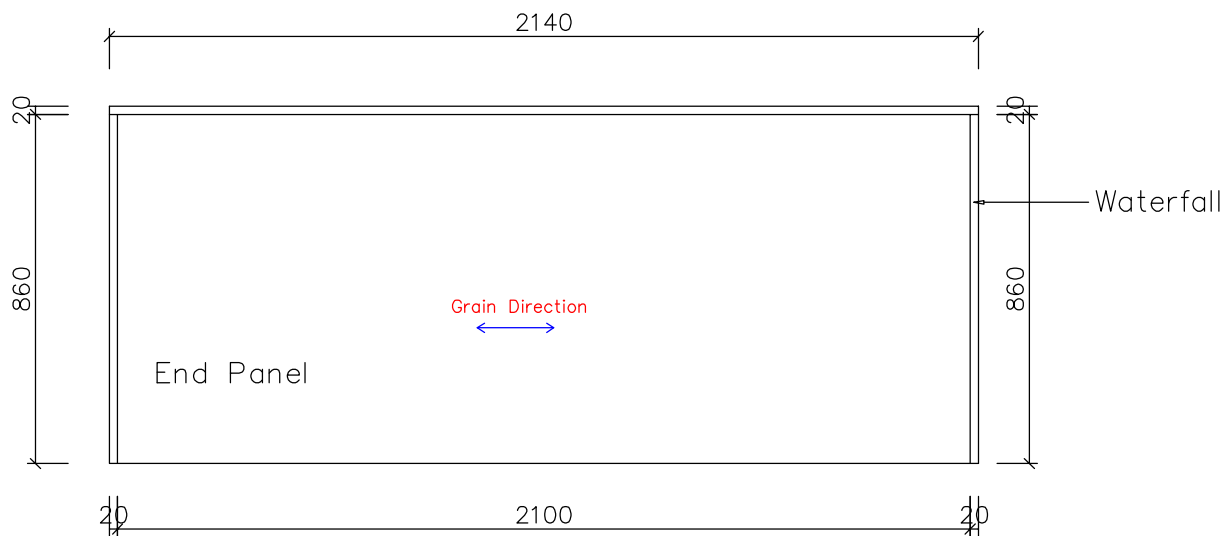
Elevation D
