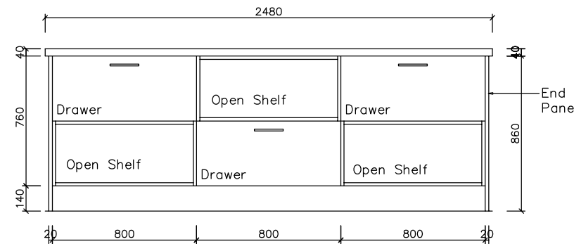
Elevation D
