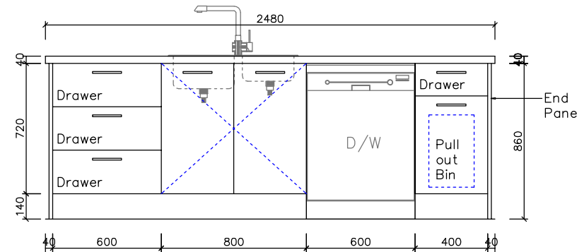
Elevation C
