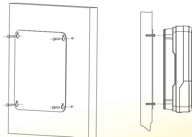
Figure 2-2 Fix the solar charge controller
