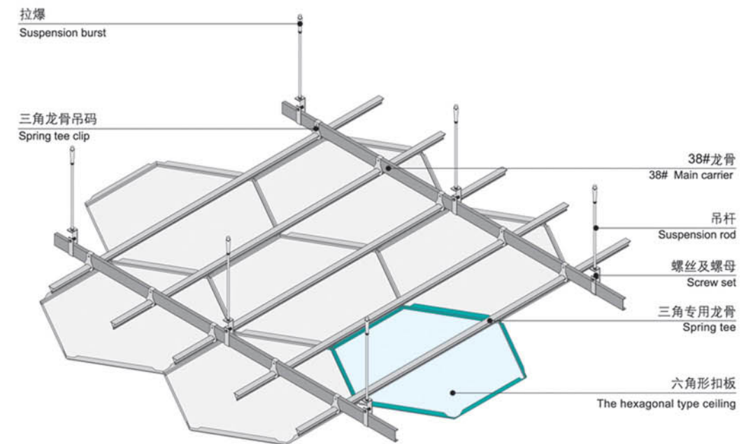
六角形扣板天花安装示意图 The hexagonal type ceiling installation diagram
