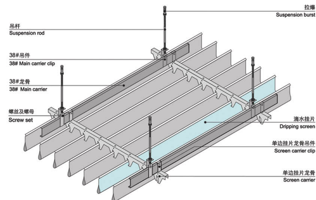
型材滴水挂片天花安装示意图 Dripping screen ceiling installation diagram
