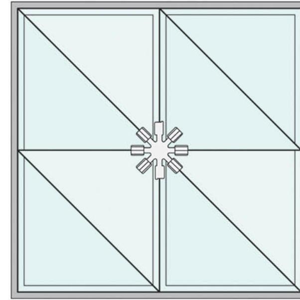
等腰三角板安装图 Triangle patent ceiling installation diagram
