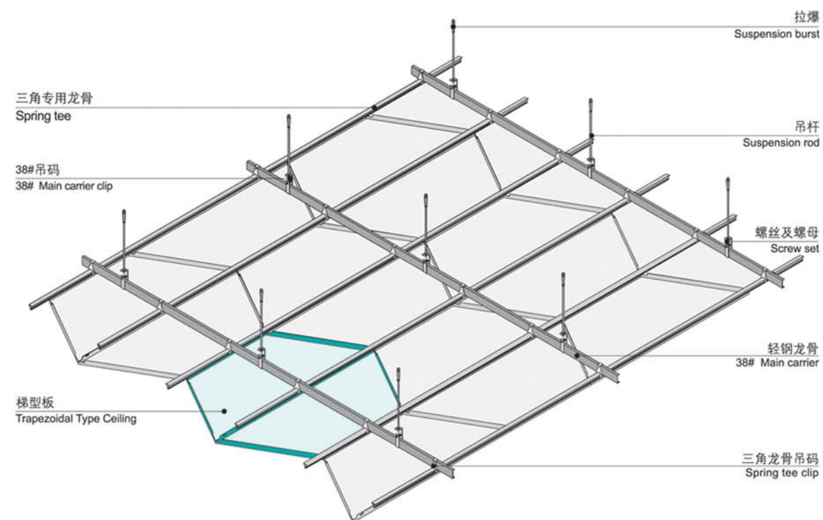
梯形扣板天花安装示意图 Trapezoidal type ceiling installation diagram
