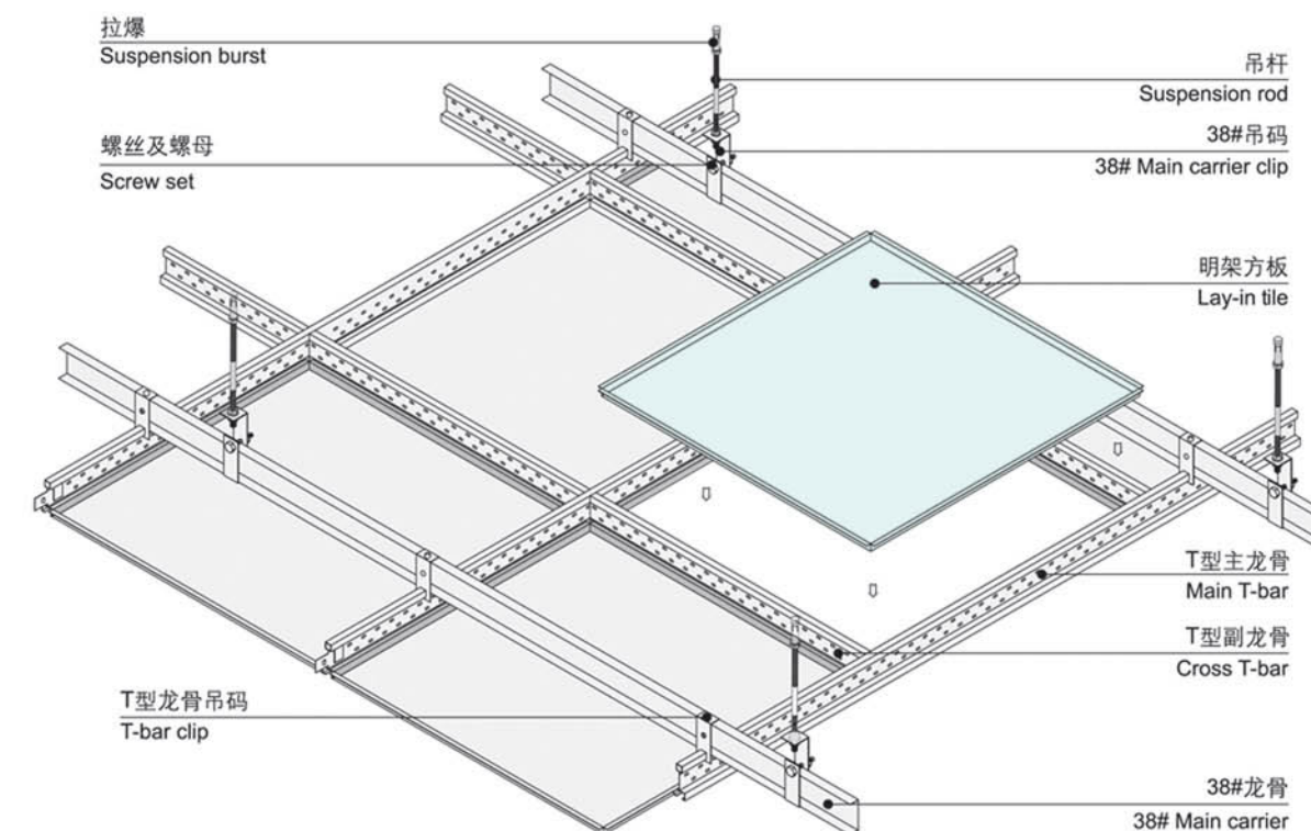
方板明架天花安装示意图 Lay-in tile ceiling installation diagram
