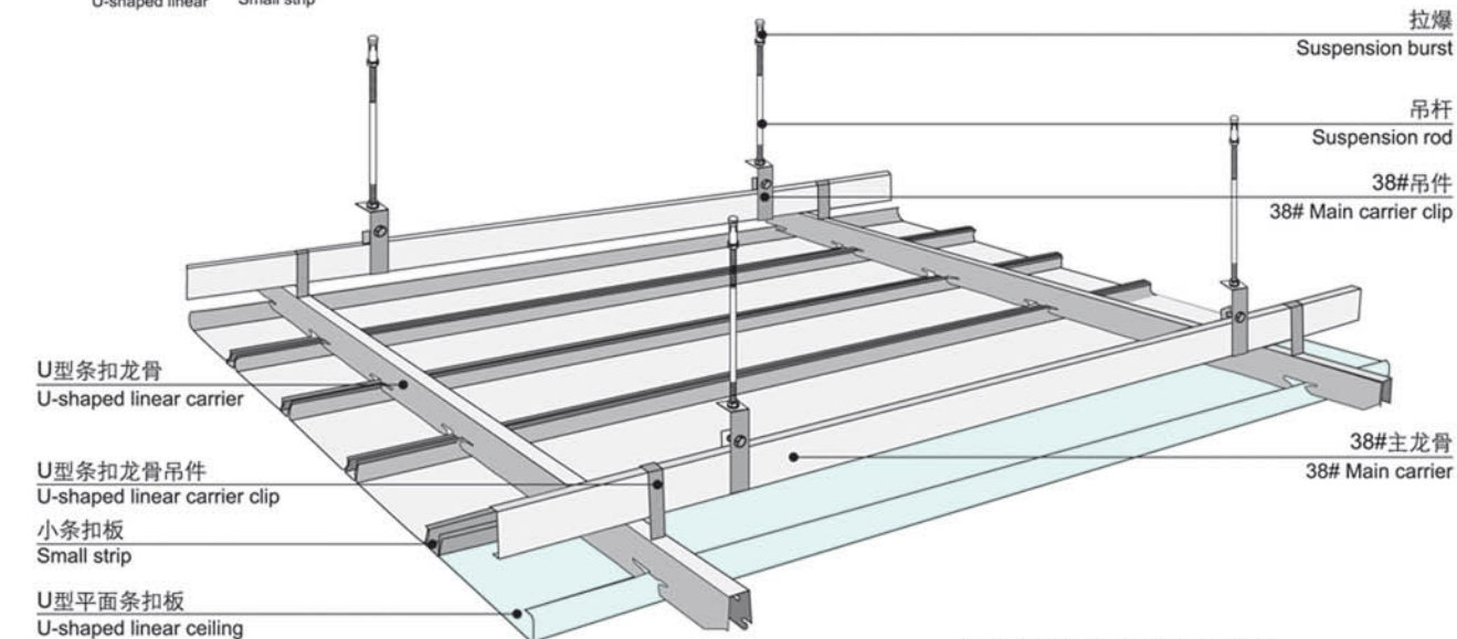
条扣配小条天花安装示意图 U-shaped linear with small strip ceiling installation diagram
