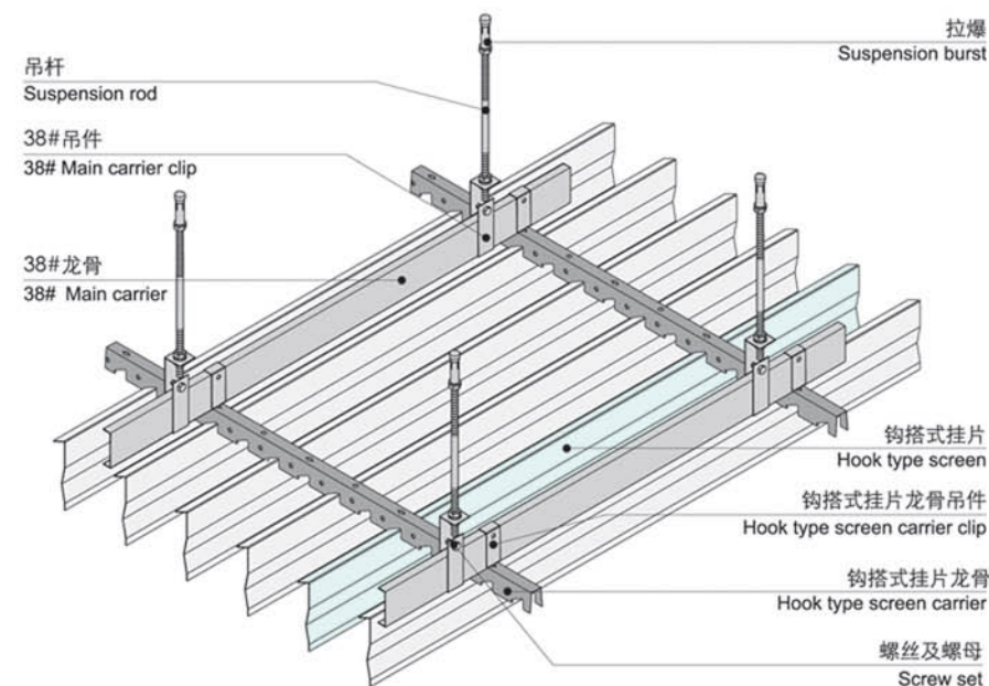
钩搭式挂片天花安装示意图 Hook type screen ceiling installation diagram
