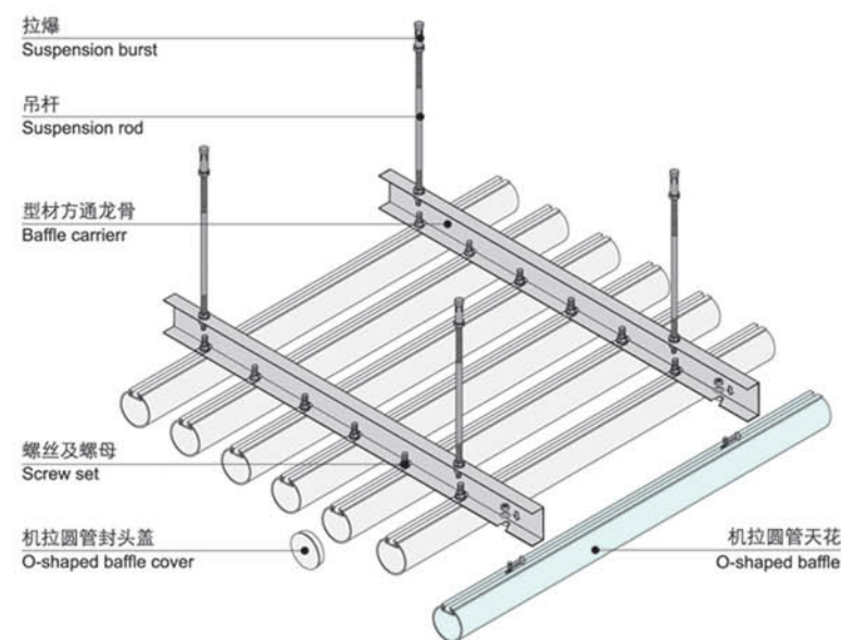
机拉圆管天花安装示意图 O-Shaped baffle ceiling installation diagram
