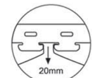
20mm 留缝 With 20mm gap
