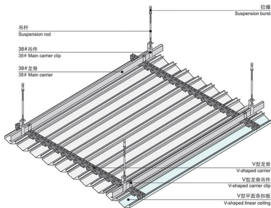
V型条扣天花安装示意图 V-shaped linear ceiling installation diagram
