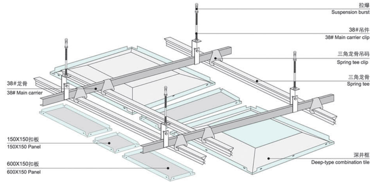
深井型组合板天花安装图 Deep-type combination ceiling installation diagram
