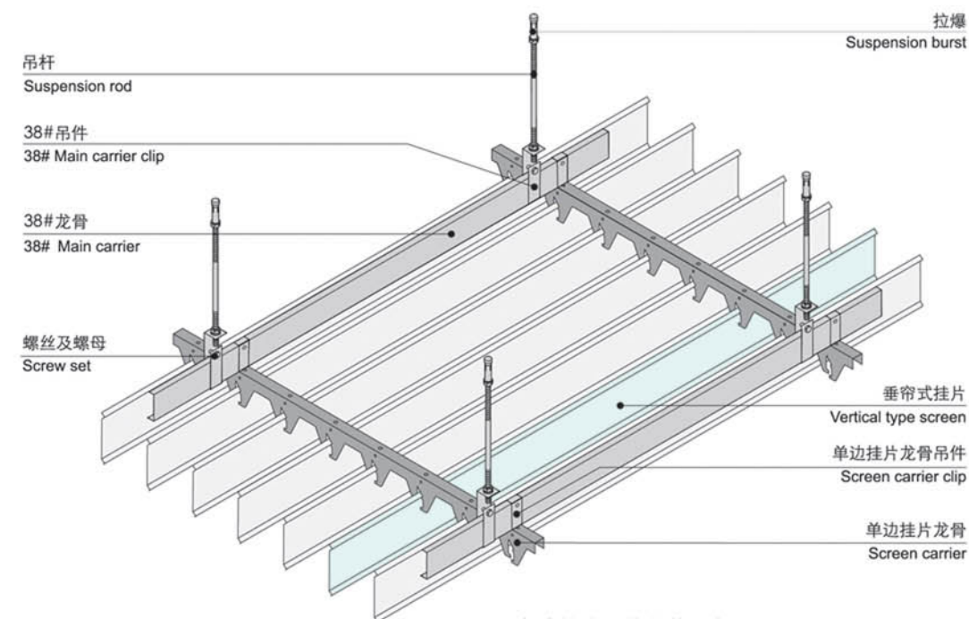
垂帘式挂片天花安装示意图 Vertical type screen ceiling installation diagram
