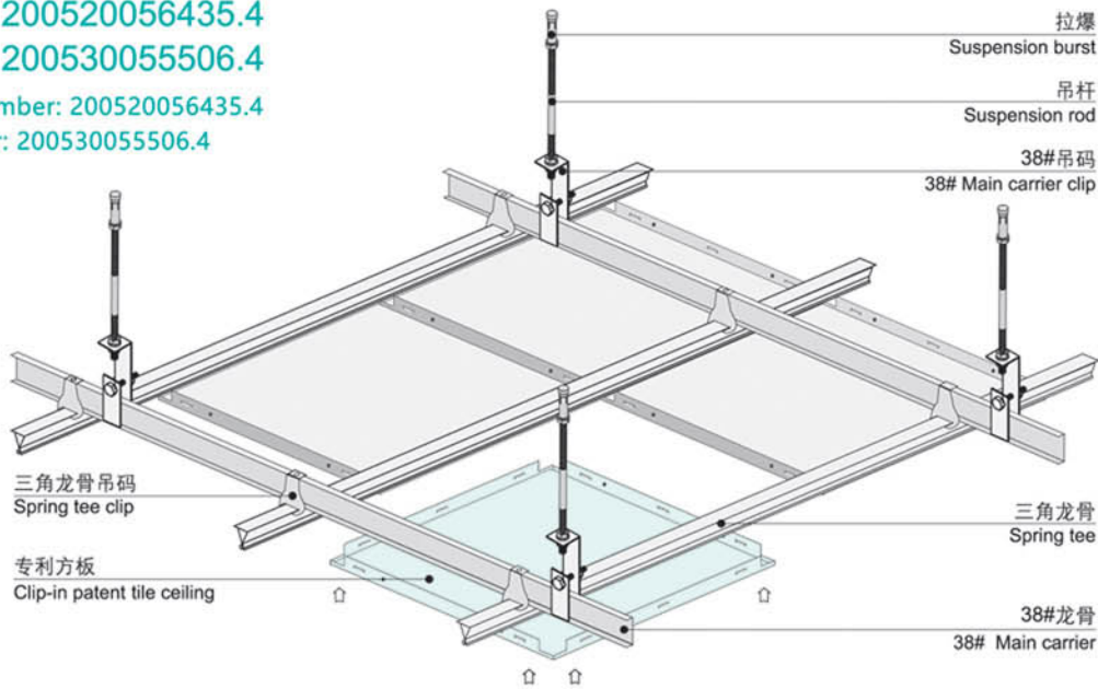
专利方板天花安装示意图 Clip-in patent tile ceiling installation diagram
