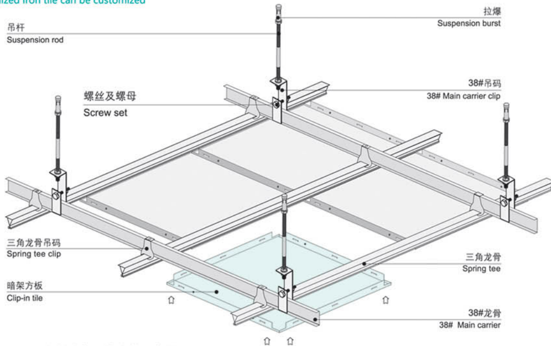
方板暗架天花安装示意图 The installation of clip-in tile ceiling system
