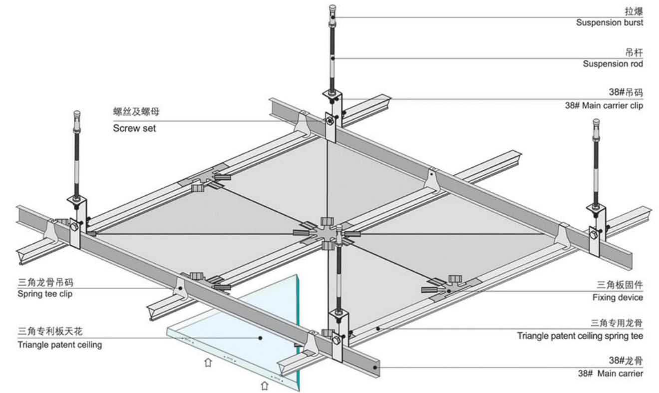
等腰三角板安装图 Triangle patent ceiling installation diagram
