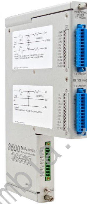
Prox/Seismic Internal Barrier I/O Module
