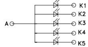
BL CIRCUIT DIAGRAM
