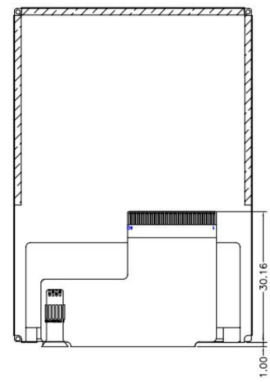
AFTER BENDING FPC FPC折弯后示图
