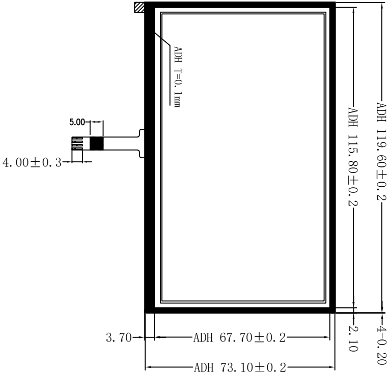
Back view
